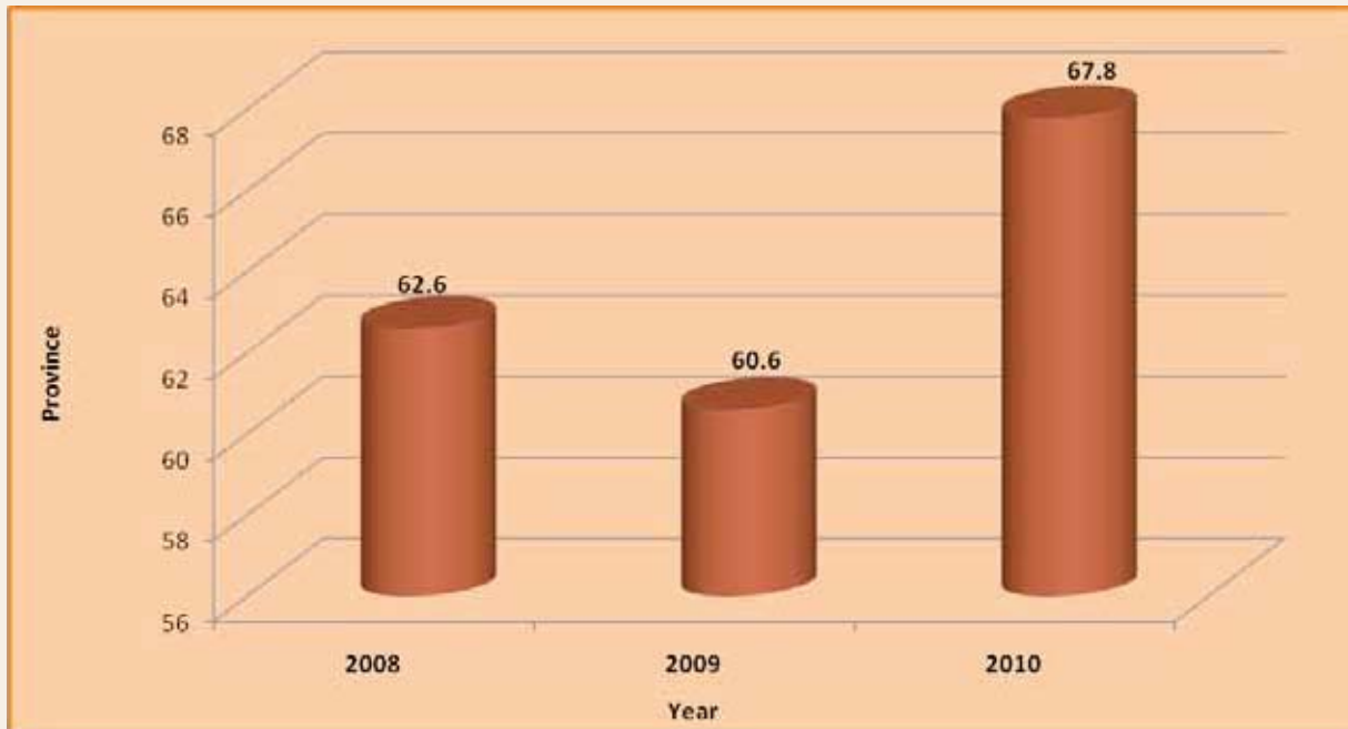
Figure 8: NSC performance: 2008 – 2010
