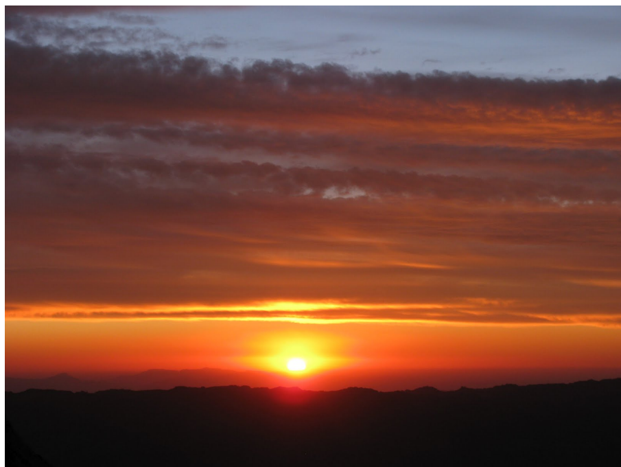
Living things need light energy from the Sun to survive.
