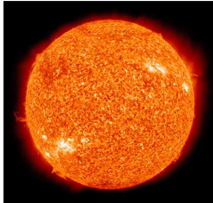
The Sun photographed by NASA.
