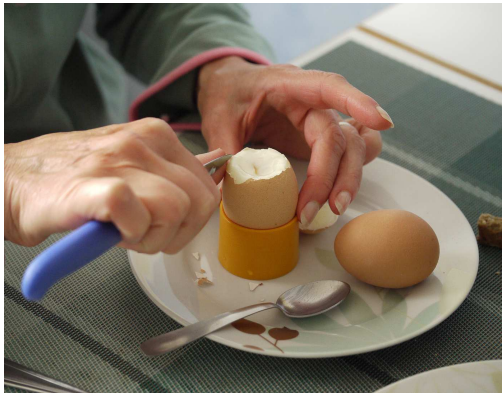
Energy is stored in food, such as eggs, which we eat for breakfast.
