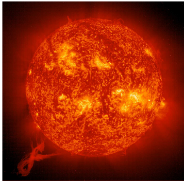
The Sun looks like this through a special camera. Never look at the Sun with just your eyes.
