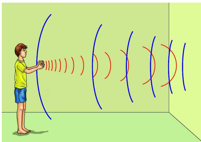
An echo occurs when sound bounces back off a surface and you hear it again.
