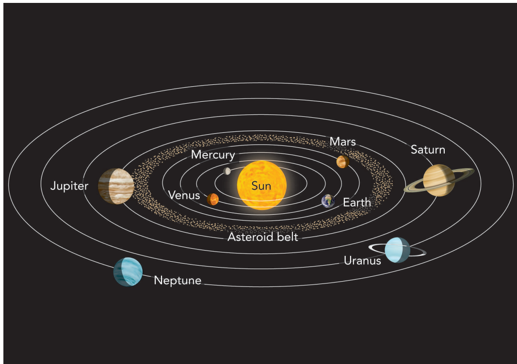
Drawing of the planets orbiting around the Sun. The planets are really much further away and much smaller than you see here.
