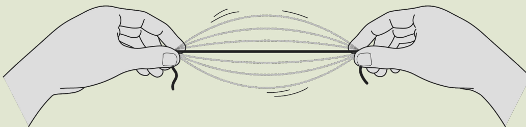
The elastic makes a sound when it moves.
