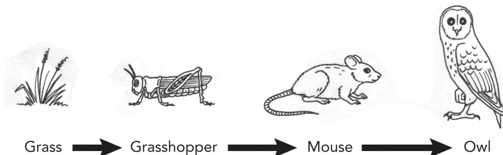
An example of a food chain
