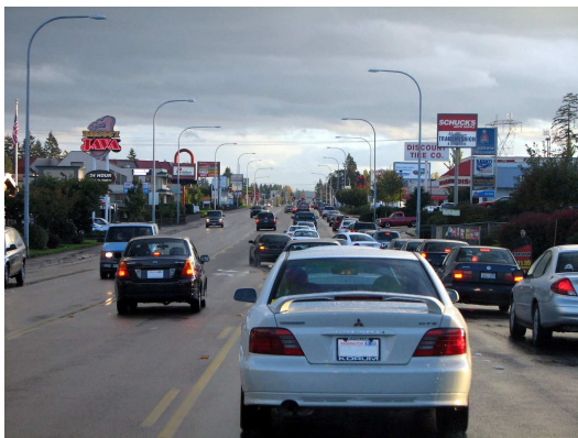
We use petrol or diesel to drive our cars.
