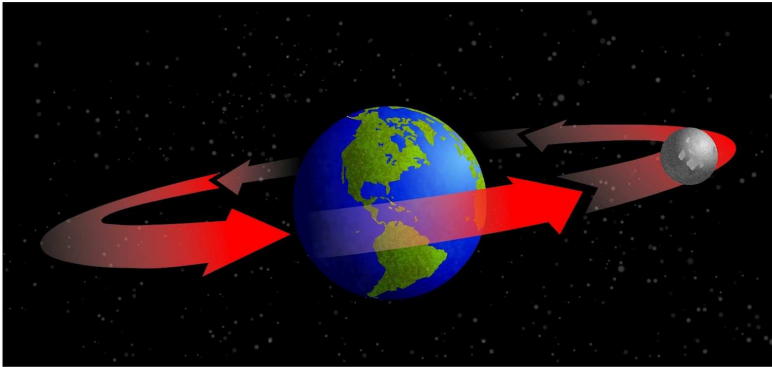
The Moon orbits the Earth once every 29\frac{1}{2} days.
