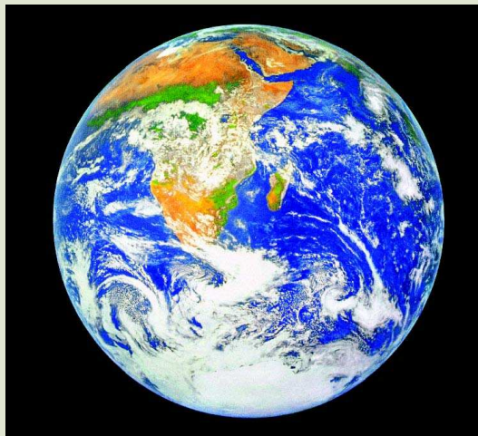
Planet Earth: this is what it looks like from a spacecraft very far above the ground.
