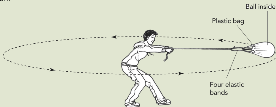
The ball orbits in a circle path around the learner.
