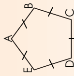
Pentagoon
