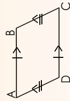
Parallelogram
