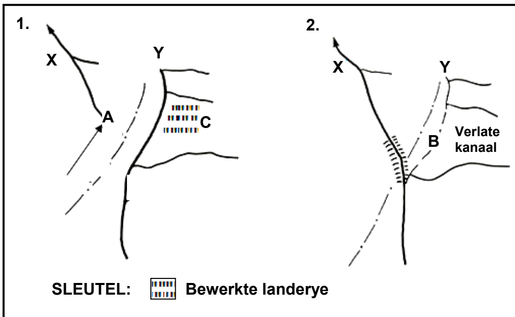
FIGUUR 2.6: STROOMROOF
