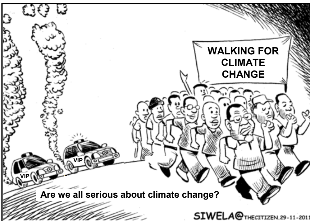
FIGURE 1.4: CLIMATE CHANGE
