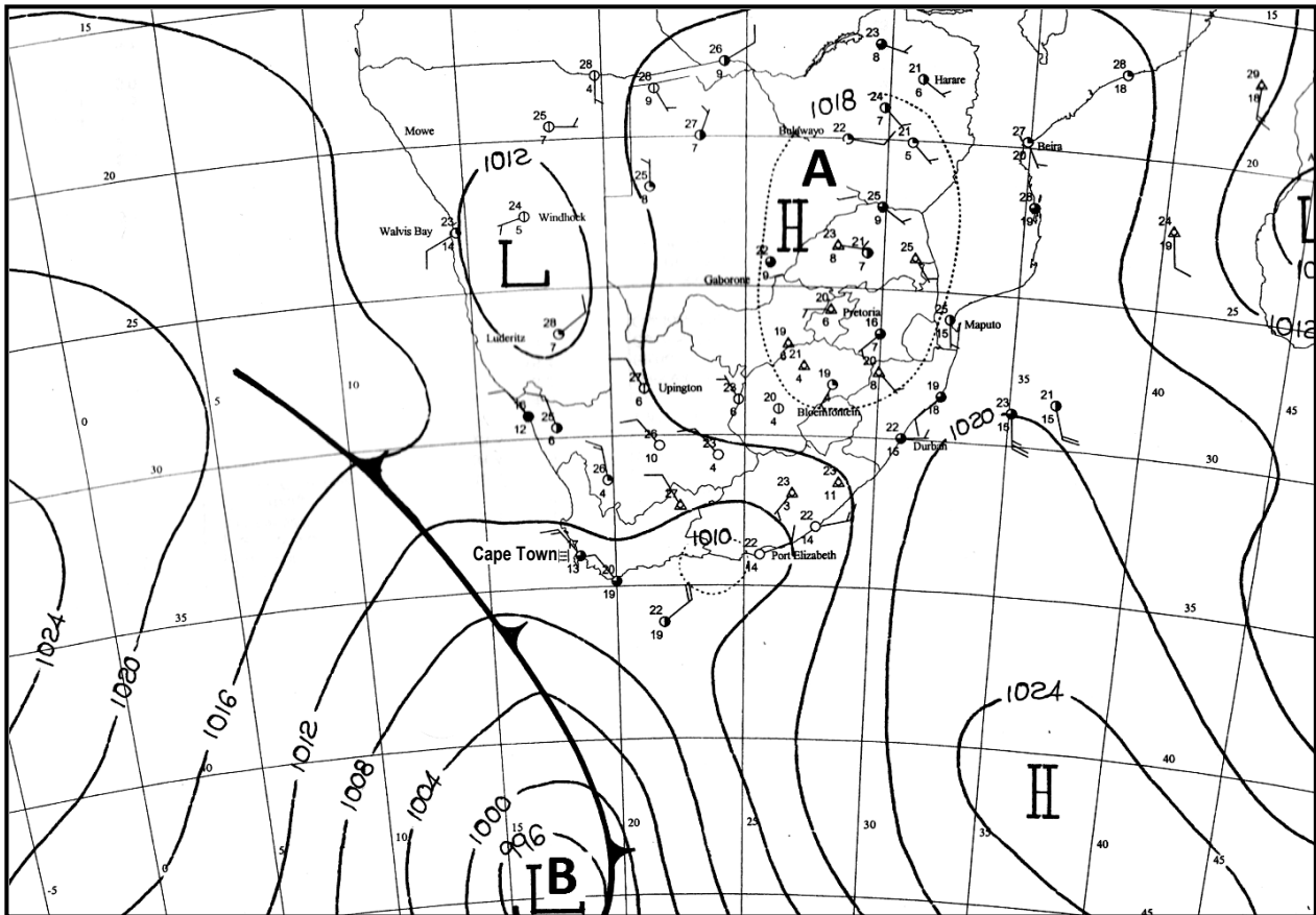
FIGURE 1.3: SYNOPTIC WEATHER MAP
