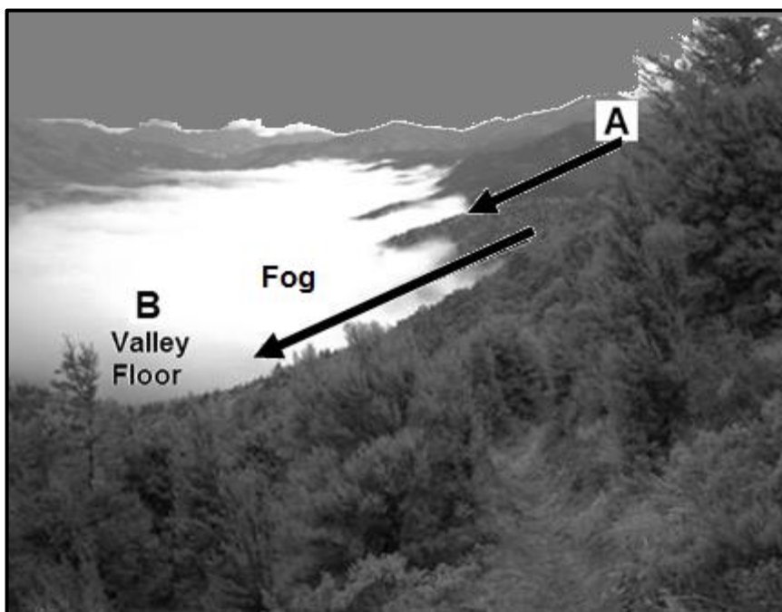
FIGURE 1.4: A KATABATIC WIND
