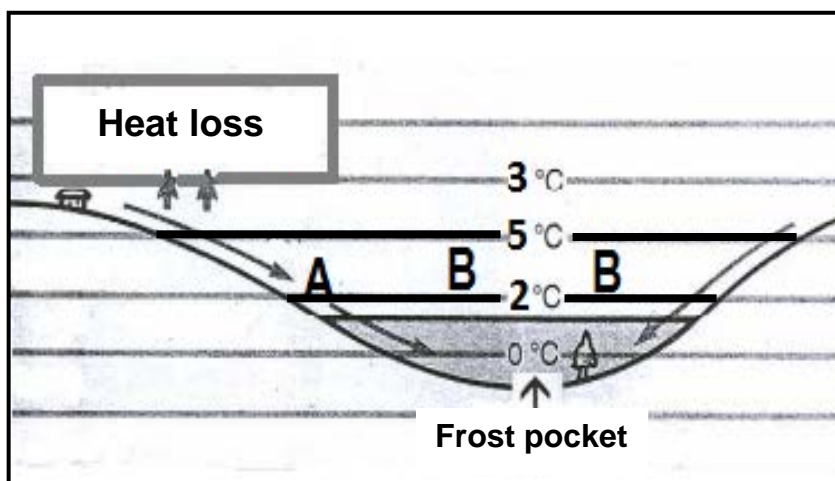
FIGURE 2.4: VALLEY CLIMATES
