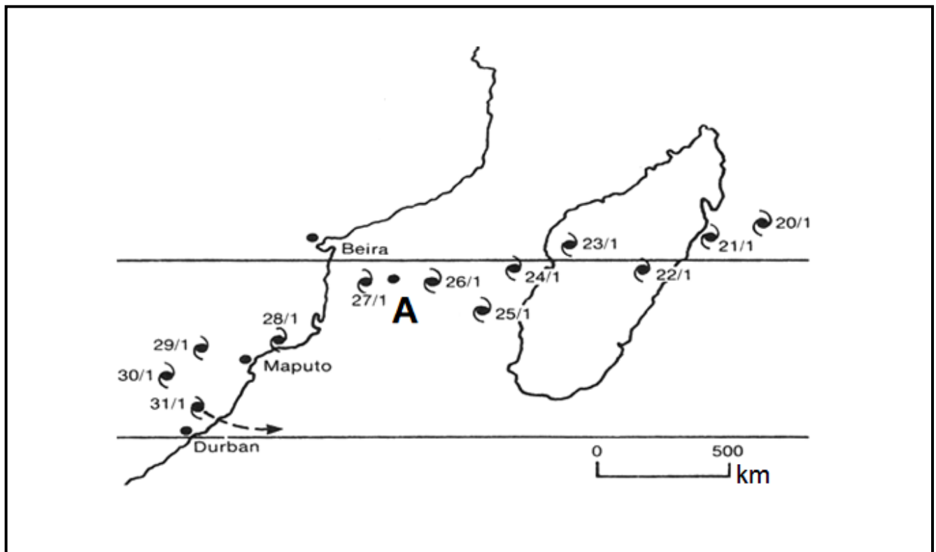
FIGURE 2.3: TROPICAL CYCLONE
