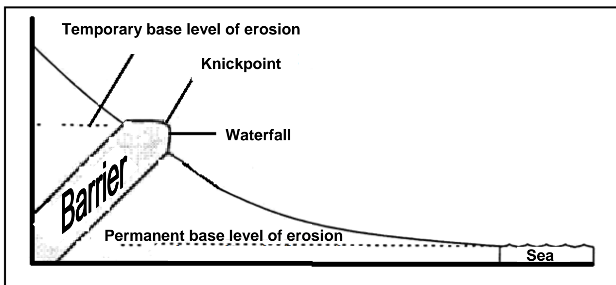
FIGURE 2.2: RIVER PROFILE
