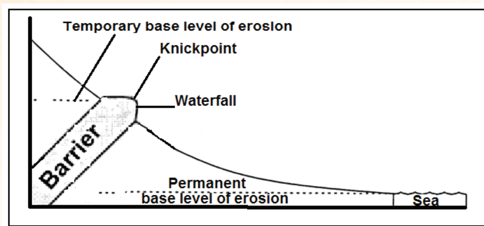
FIGURE 7.2: RIVER PROFILE
