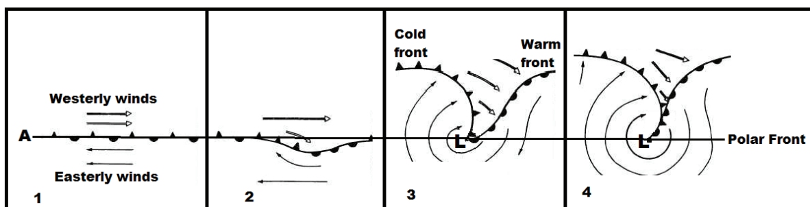
FIGURE 1.2: STAGES IN THE DEVELOPMENT OF A MID-LATITUDE CYCLONE
