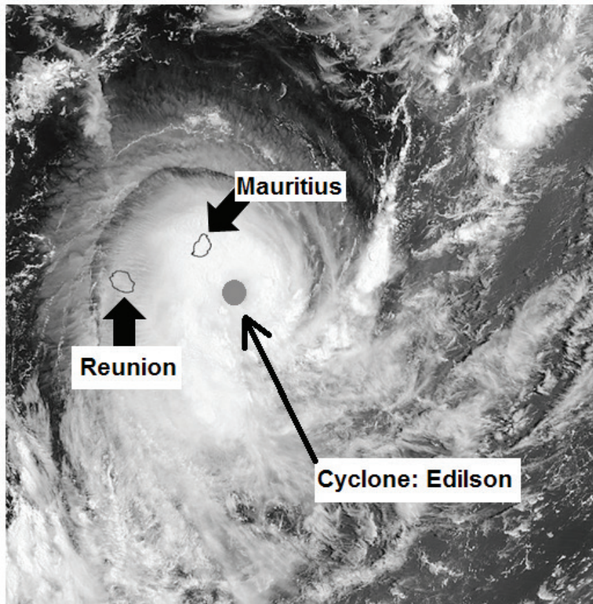
FIGURE 2.1: SATELLITE IMAGE OF A TROPICAL STORM
