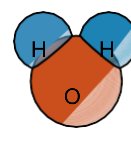
Water, H_2O .
