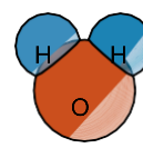
Water, H_2O .
